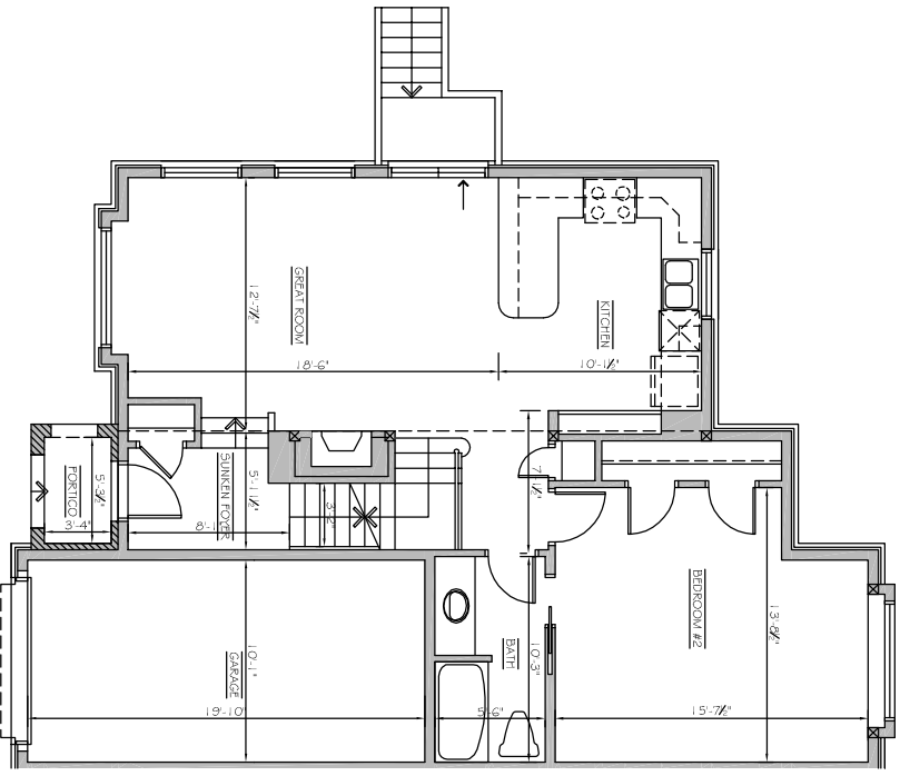
1 GROUND FLOOR PLAN SCALE: 3/32" = 1'-0"
