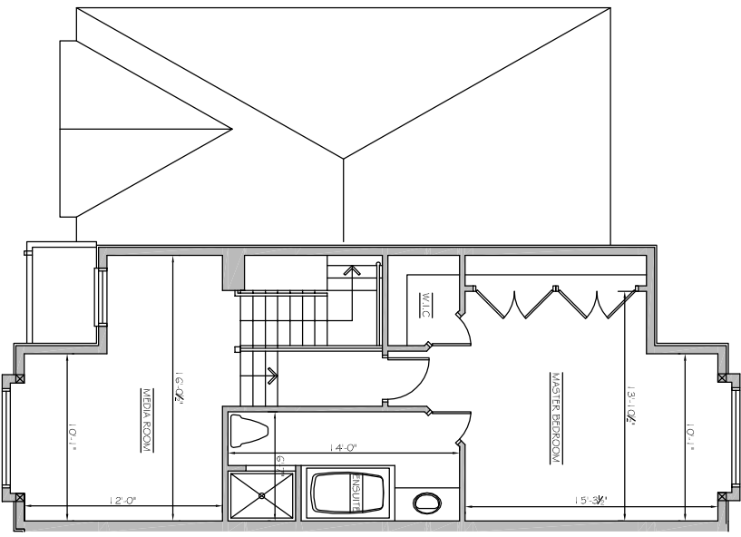
2 UPPER FLOOR PLAN SCALE: 3/32" = 1'-0"
